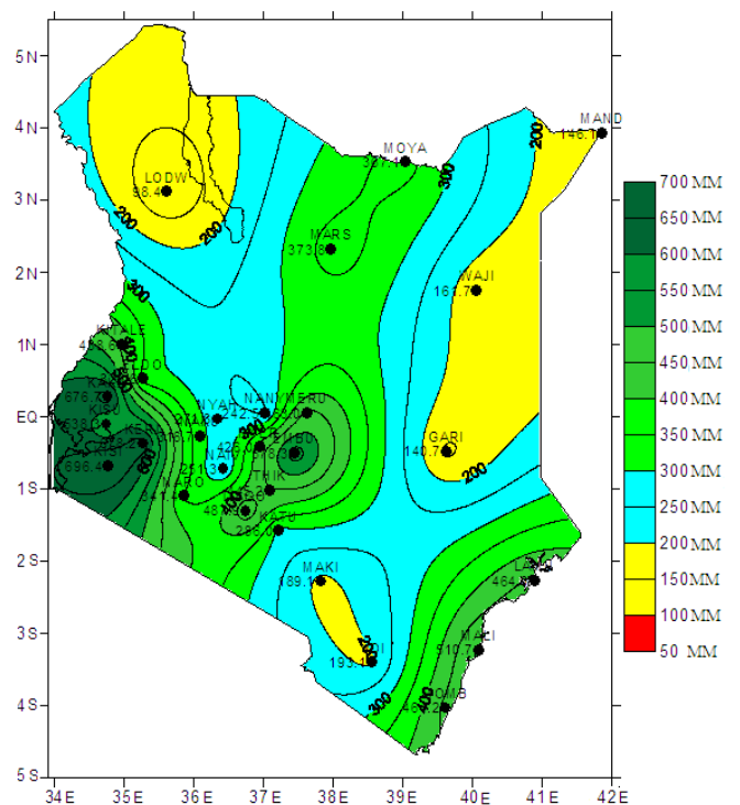
FIG. 2: MEAN MARCH-MAY SEASONAL RAINFALL
