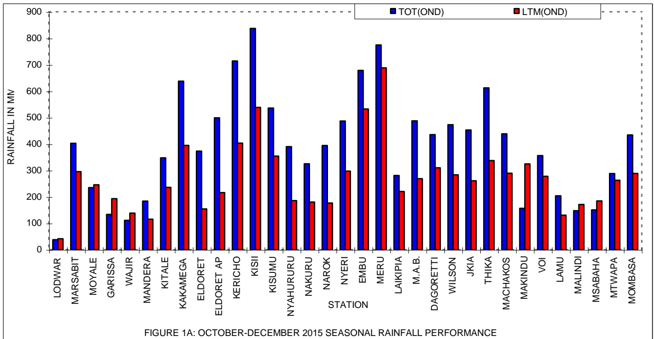
FIGURE 1A: OCTOBER-DECEMBER 2015 SEASONAL RAINFALL PERFORMANCE
