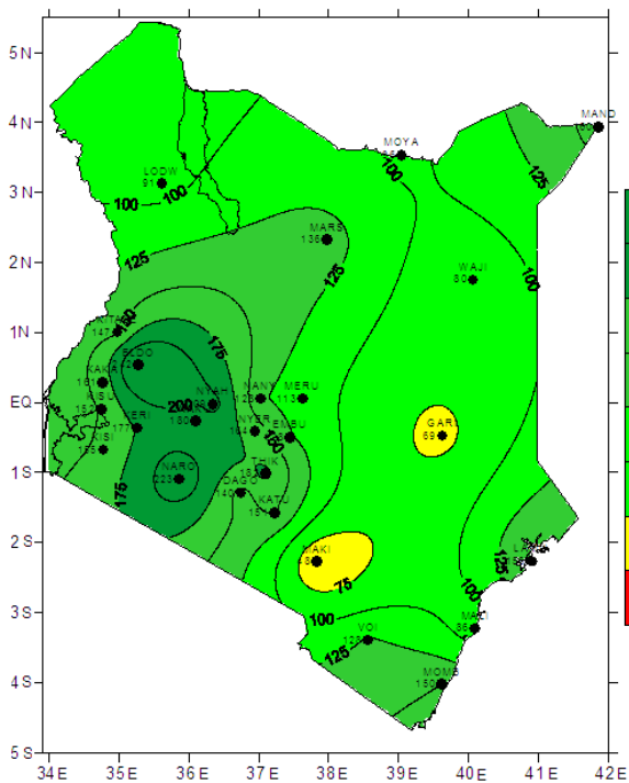
FIGURE 1B: OND 2015 RAINFALL DISTRIBUTION IN KENYA
