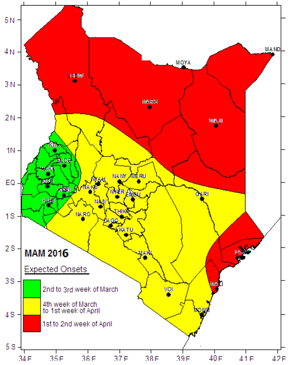
FIG. 3A: EXPECTED ONSET DATES MARCH-MAY 2016 SEASONAL RAINFALL ONSET
